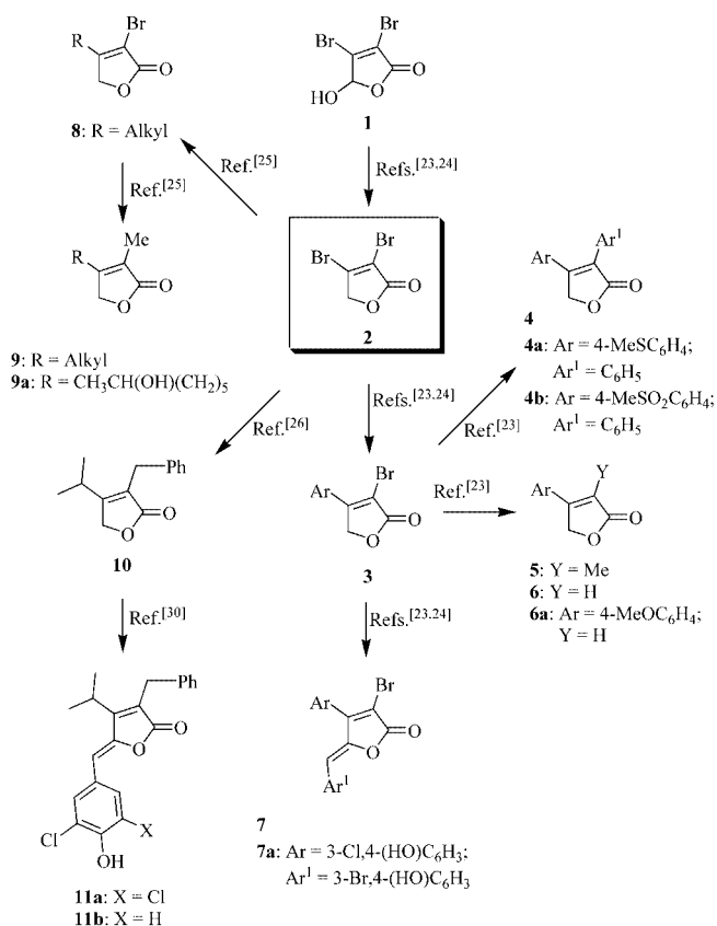
Figure 1. Chemical structures of compounds 2 , 3 , 4 , 4a , 5 , 6 , 6a , 7 , 7a , 8 , 9 , 9a , 10 , 11a and 11b prepared from mucobromic acid ( 1 )
